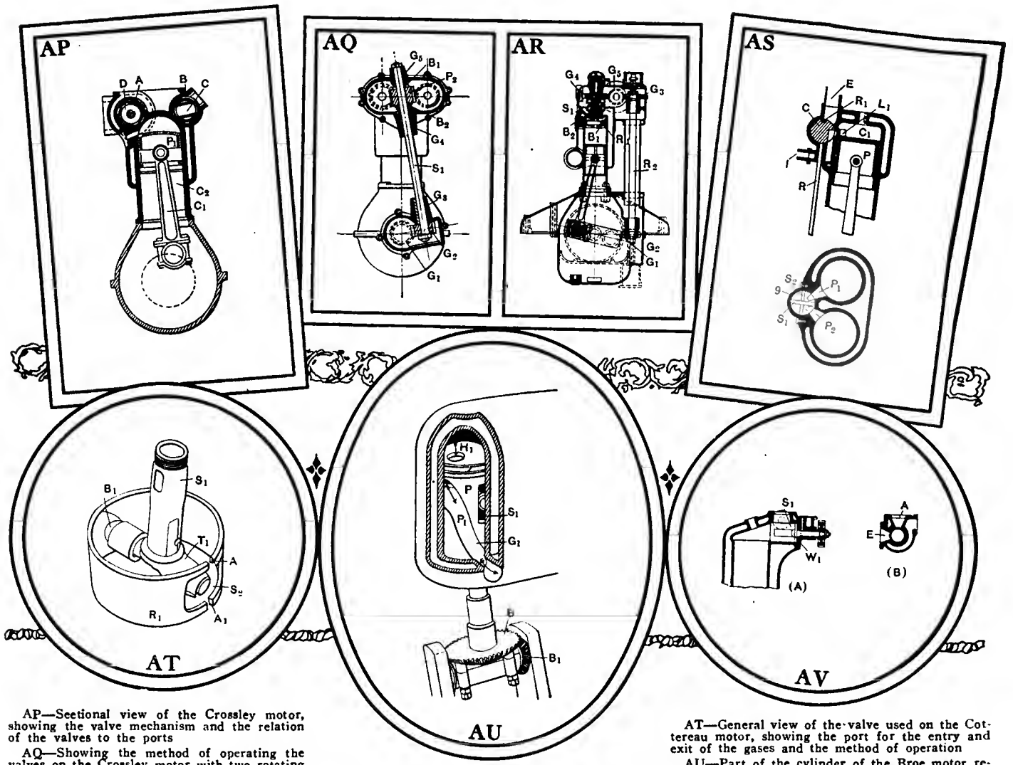
AS—Transverse sectional view of Wridgway motor in which a sphere suitably slotted is employed to control gases. Plan view shows relation of sphere to the cylinder ports
